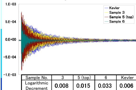
Vibration damping: Kevlar comparison
